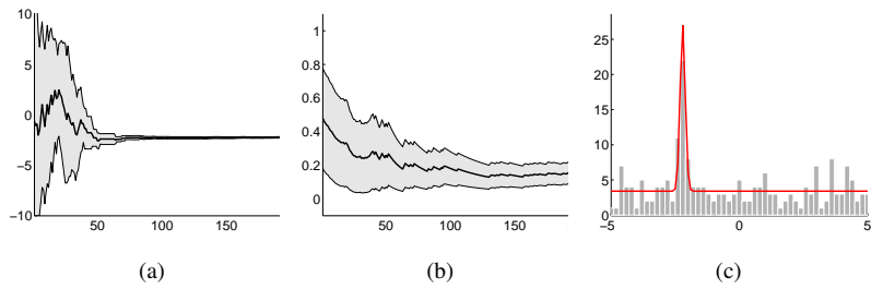
Figure 4: Parametric update evolution The first two plots show the evolution of the depth estimate Z and the inlier probability \pi . We show the mean \pm two standard deviations. The third plot shows the measurement histogram superimposed with the measurement posterior p(x|x_1, \dots, x_n) . Both the mean and the outlier level have been correctly captured.
