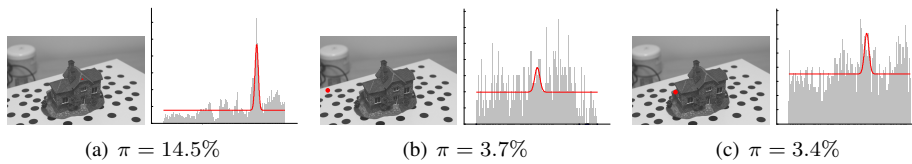
Figure 5: Three types of pixel sensors These figures show the measurement histograms and the superimposed measurement posterior p(x|x_1, \dots, x_m) for three types of pixel sensor. In (a) the pixel is a well-textured point on the object. In (b) the pixel corresponds to a completely untextured white point on the ground. In (c) the pixel corresponds to a point that will get occluded within the next few frames. The estimated inlier ratio is shown in the three cases. The two pathological cases, (b) and (c), can be identified from their low inlier ratio.
