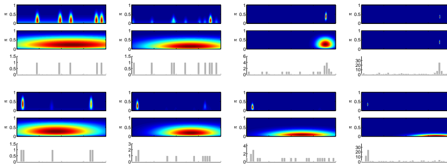
Figure 3: Non-parametric vs. parametric modeling of posterior distribution. The first row shows the posterior distribution that is modeled non-parametrically as a 2d histogram. The four columns represent four time instances (after 5, 10, 20 and 100 updates). The second row shows the evolution of our parametric Gaussian \times Beta approximation. Even though our model cannot capture the multi-modal nature of the true posterior, after a few iterations it converges to the same point estimate. The third row shows the histogram of measurements that have been seen by the system in each time instance. The last three rows show one of the few cases where the parametric model cannot follow the non-parametric one. When this happens it can be detected because the parametric posterior predicts a very low inlier ratio. We can therefore safely discard it. The x axis denotes depth along optic ray for all images.
