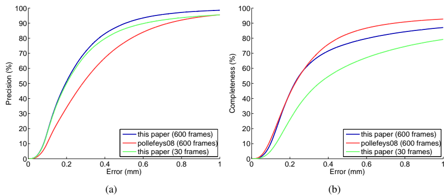
Figure 7: Accuracy and completeness curves for ground truth experiment. (a) shows accuracy results for our algorithm running in 30 and 600 frames of a video sequence of a house. The graph shows for a given distance d , how much of the reconstructed model falls within d of the ground truth. (b) measures completeness. I.e. for a distance d how much of the ground truth falls within d of the reconstructed model. Our results are more accurate but somewhat less complete. This is because our method performs no regularization and returns an unmeshed point-cloud.
