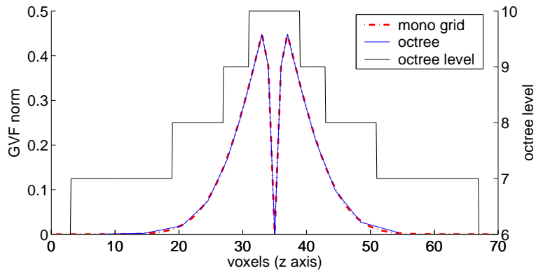
Figure 2.24: mono grid vs. octree grid GVF with \mu = 0.1 .
