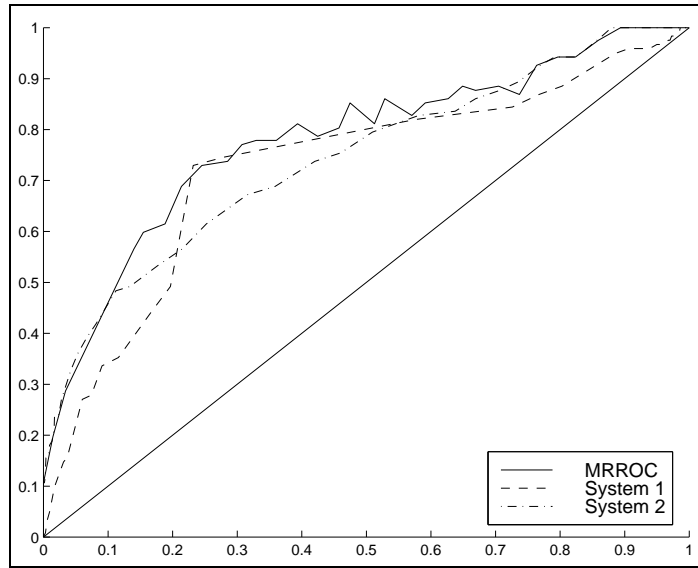
Figure 9: The MRROC plotted for the Unseen data set. The MRROC is consistent with that predicated by the convex hull over the Test data ROC curves. The ROC curves for System 1 and System 2 using the Unseen data are plotted for comparison with the MRROC .
