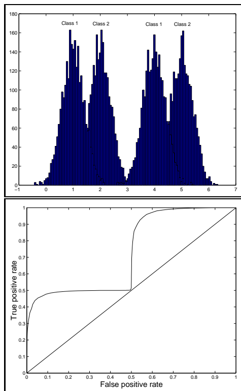
Figure 4: Top: an example of 2 class multi modal data. This data will present problems to linear classification systems. Bottom: the ROC curve produced by varying the threshold on the output of a linear model of the multi modal data shown. The ROC has a step like appearance because the linear model fails to capture the nature of the data.
