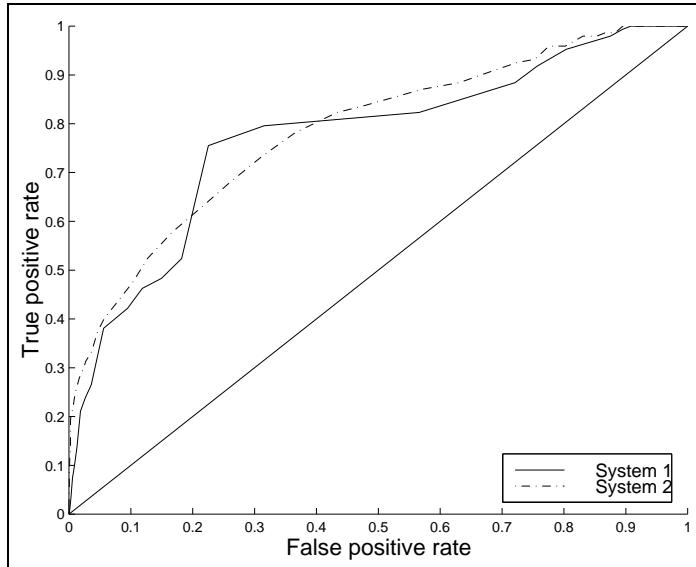
Figure 7: The ROC curves for both classification systems using the thyroid Test data.
