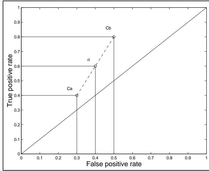
Figure 3: An example of a realisable classifier. The point r_i on the line joining c_a and c_b may be realised by the application of Theorem 1
