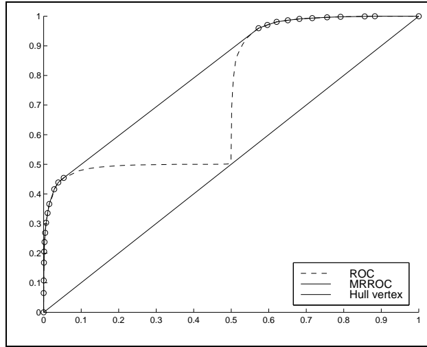
Figure 5: The convex hull containing the ROC of a linear model is found. This hull is the MRROC of the set of realisable classifiers produced from the set of existing linear classifiers
