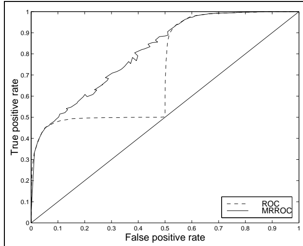
Figure 6: The MRROC plotted for an unseen data set. The MRROC is consistent with that predicted.
