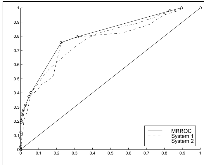
Figure 8: The convex hull over both original ROC curves. This is the predicted MRROC .
