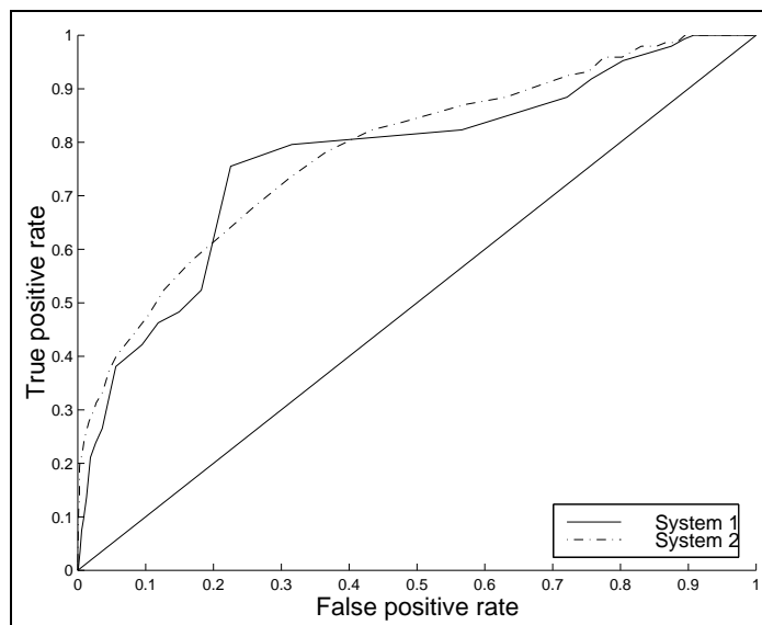
Figure 2: The ROC curves of two classification systems cross.
