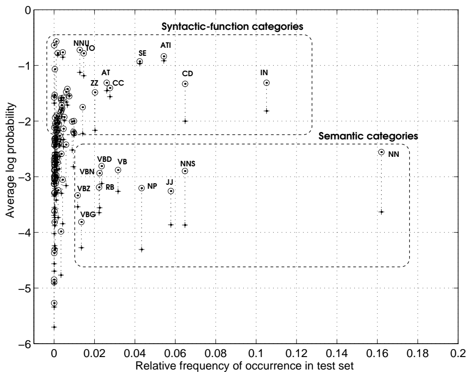
Figure 3.12: Average log probability per category for both word-based (⊙) and category-based (+) models.
