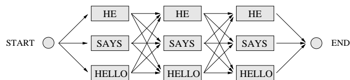
Figure 6.2: The search space when using a bigram language model.
