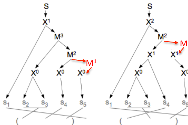
Figure 11 Movement allowed by two grammars: shallow-1, with K_1 = 1 , K_2 = 3 [left], and shallow-2, with K_1 = 1 , K_2 = 3 [right]. Both grammars allow movement of the bracketed term as a unit. Shallow-1 requires that translation within the object moved be monotonic while shallow-2 allows up to two levels of reordering.
