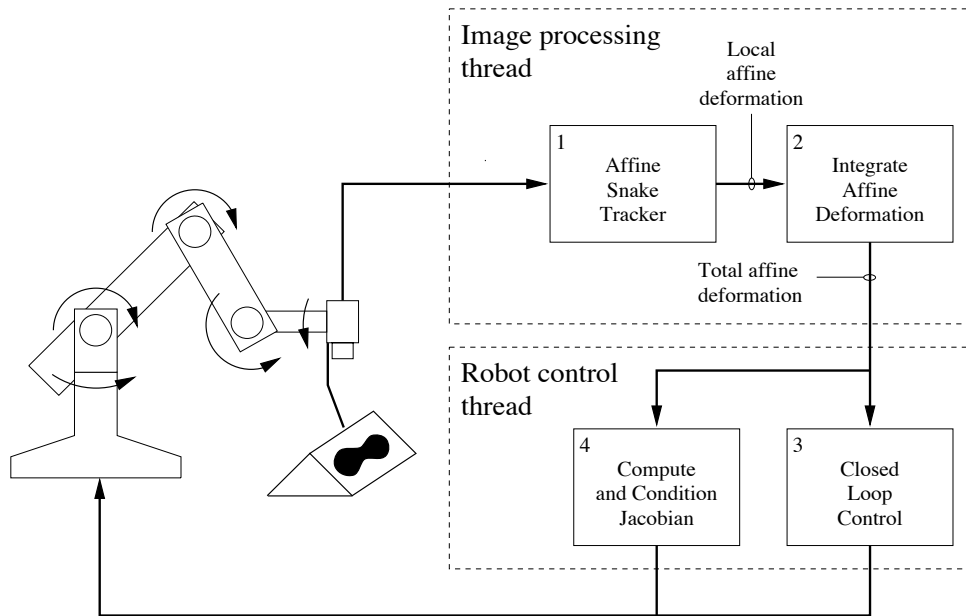
Fig. 2. System architecture
