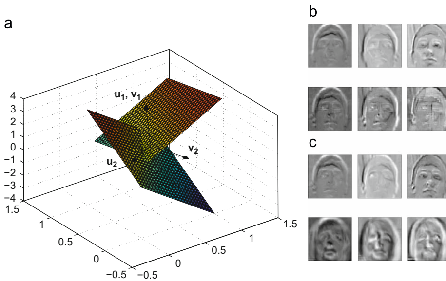
Fig. 3. An illustration of the concept of principal angles and principal vectors in the case of two 2D subspaces embedded in a 3D space. As two such subspaces necessarily intersect, the first pair of principal vectors is the same (i.e. \mathbf{u}_1 = \mathbf{v}_1 ). However, the second pair is not, and in this case forms the second principal angle of \cos^{-1} \rho_2 = \cos^{-1}(0.8084) \approx 36^\circ . The top three pairs of principal vectors, displayed as images, when the subspaces correspond to image sets of the same and different individuals are displayed in (b) and (c) (top rows corresponds to \mathbf{u}_i , bottom rows to \mathbf{v}_i ). In (b), the most similar modes of pattern variation, represented by principal vectors, are very much alike in spite of different illumination conditions used in data acquisition.
