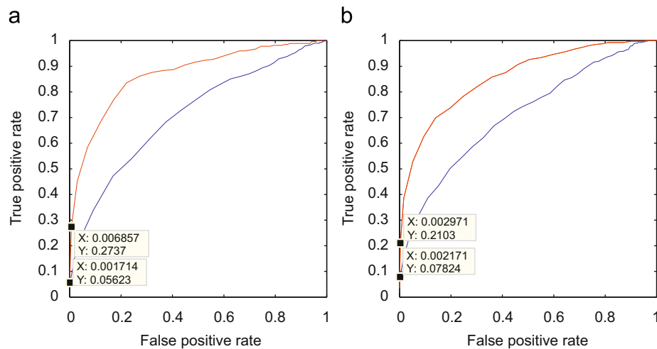
Fig. 14. Isolated local features receiver-operator characteristics (ROC): for visual (blue) and thermal (red) spectra. (a) Eyes and (b) mouth. (For interpretation of the references to color in this figure legend, the reader is referred to the web version of this article.)
