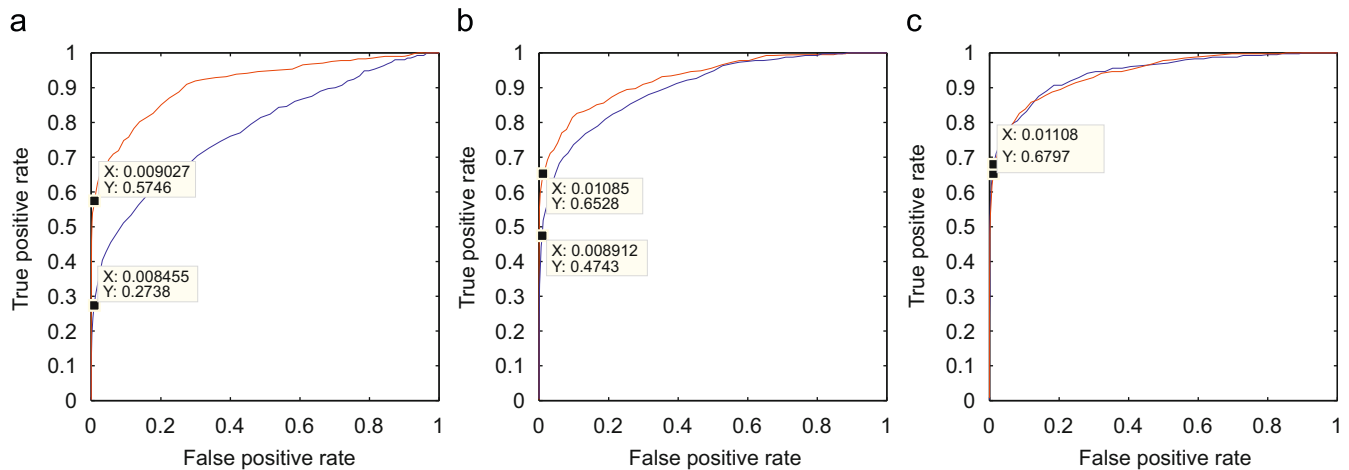
Fig. 15. Holistic representations receiver-operator characteristics (ROC) for visual (blue) and thermal (red) spectra. (a) Unprocessed, (b) band-pass filtered and (c) self-quotient image filtered. (For interpretation of the references to color in this figure legend, the reader is referred to the web version of this article.)
