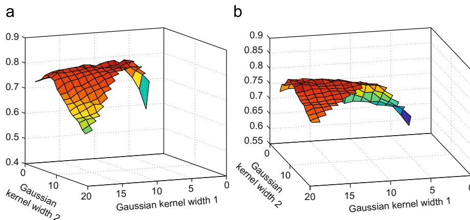
Fig. 5. The optimal combination of the lower and upper band-pass filter thresholds is estimated from a small training corpus. The plots show the recognition rate using a single modality, (a) visual and (b) thermal, as a function of the widths W_1 and W_2 of the two Gaussian kernels in (4). It is interesting to note that the optimal band-pass filter for the visual spectrum passes a rather narrow, mid-frequency band, whereas the optimal filter for the thermal spectrum is in fact a low-pass filter.
