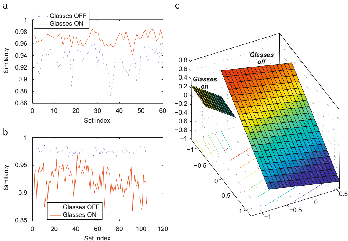
Fig. 11. (a) Inter- and (b) intra-class (glasses on and off) similarities across our data set. (c) Good discrimination by principal angles is also motivated qualitatively as the subspaces modelling appearance variations of the eye region with and without glasses on show very different orientations even when projected to the 3D principal subspace. As expected, the “glasses off” subspace describes more appearance variation, as illustrated by the proportionally greater extent of the linear patch representing it in the plot. (a) Glasses ON, (b) glasses OFF and (c) model subspaces.
