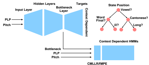
Figure 1: Language independent acoustic model.
