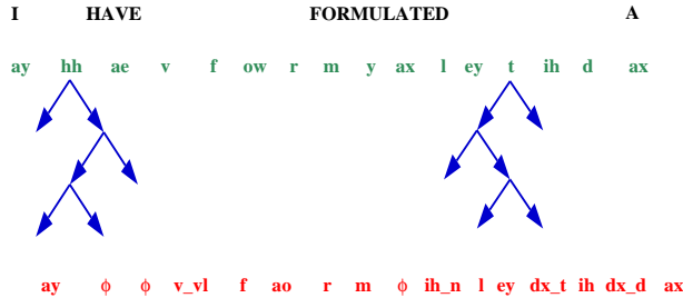
Figure 1: Decision Trees as Phone Predictors
